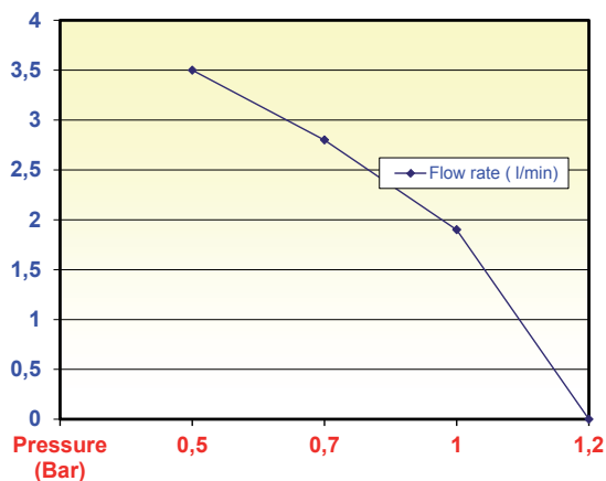
Centrifugal pump
