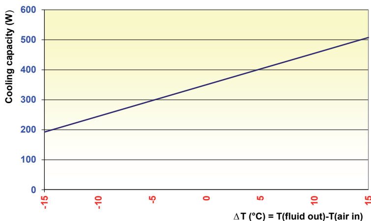
Cooling capacity
