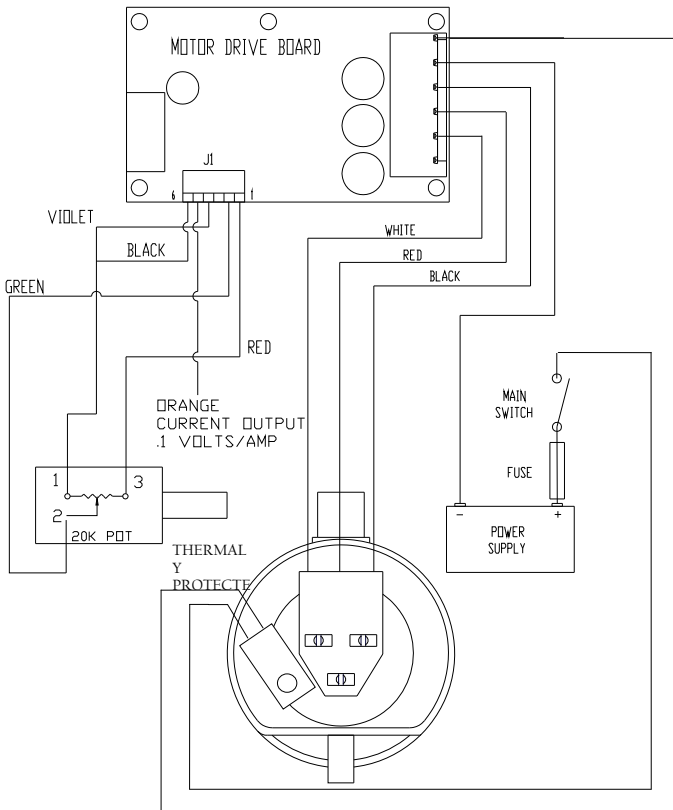
Wiring Option 1 (User supplied potentiometer)
