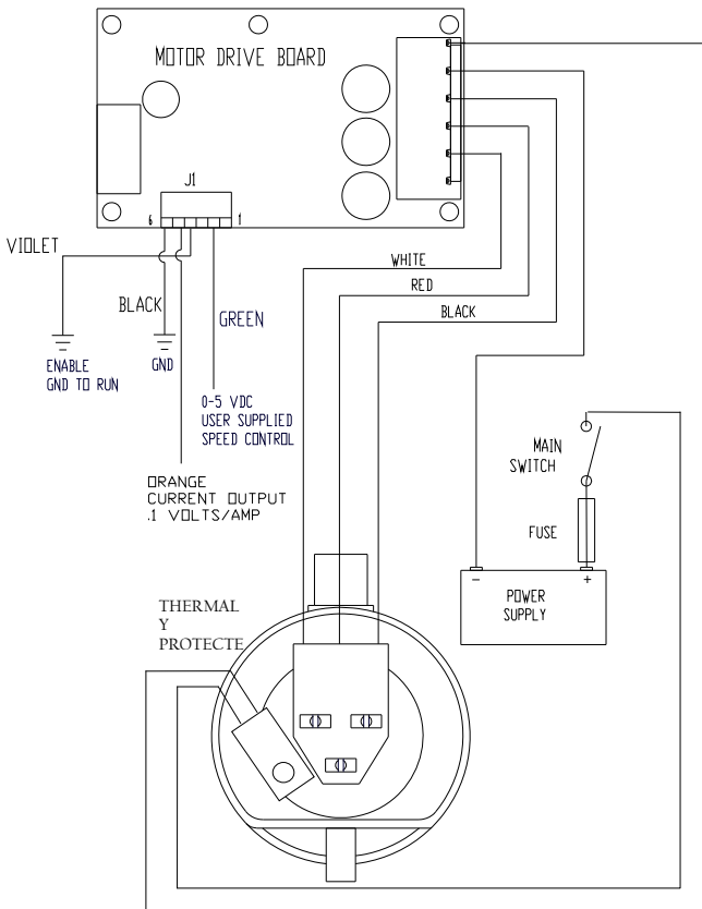
Wiring Option 2 (User supplied speed input voltage)
