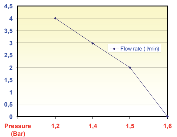
Centrifugal pump
